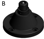
B NATO 4-hole Rigid 4 x M10 or 3/8" Bolts on 114mm PCD Base diameter 140mm Base height 100mm
