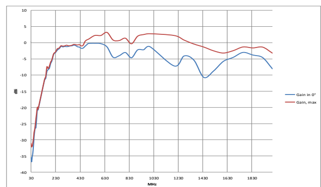
Gain (dBi)
