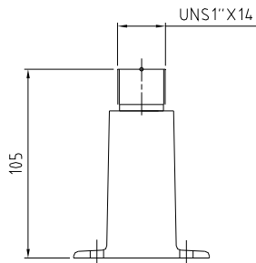
Straight-Mount Bracket
