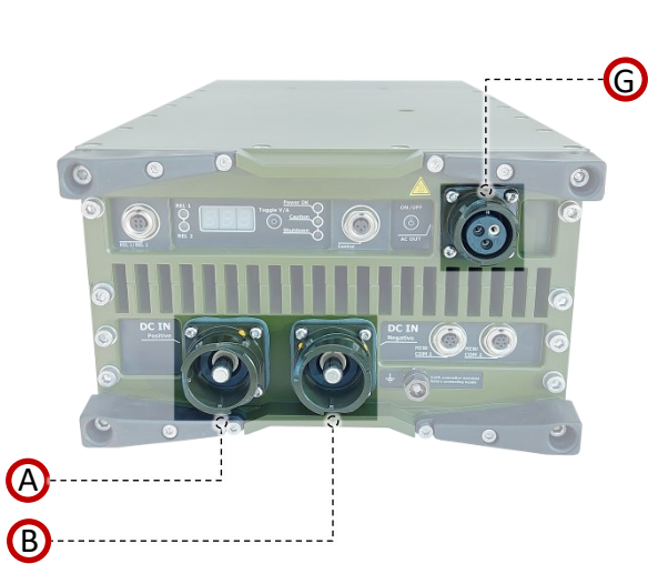
ComCompact 2000 AC/DC (Inverter) (Bayonet Connections)
