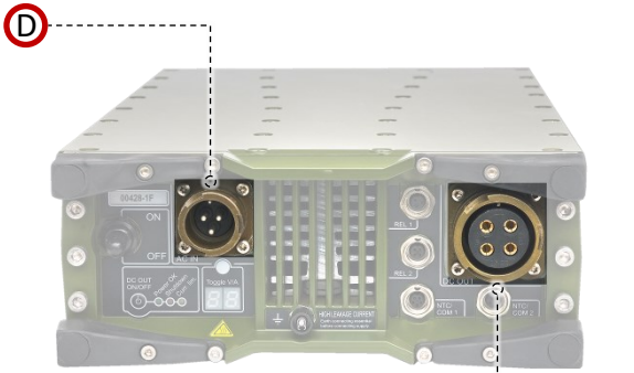
ComCompact 2400 AC/DC ComCompact 2700 AC/DC (Bayonet Connections)
