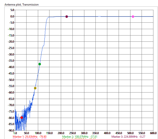
UHF 225-600 MHz
