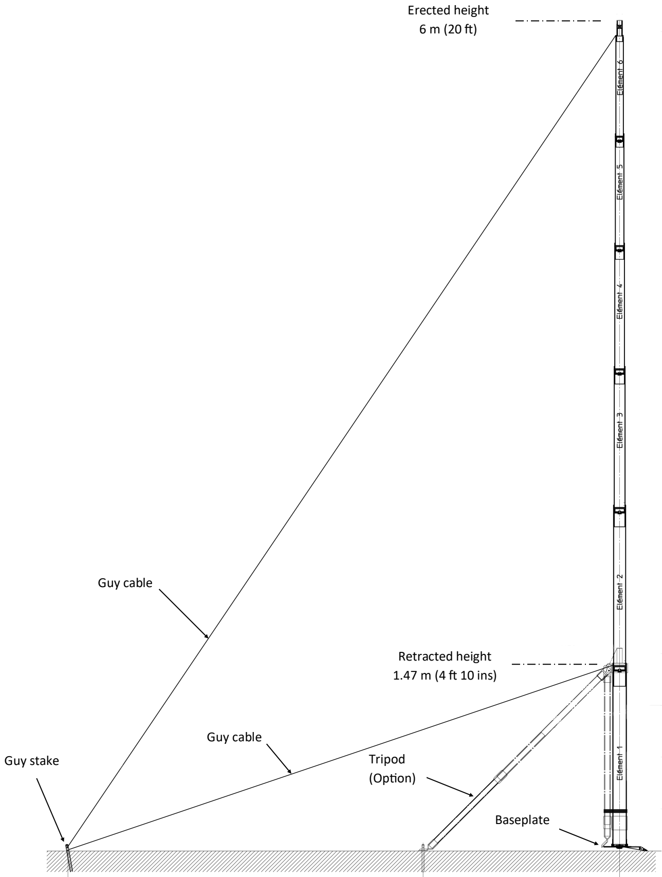
Standard installation : ground mounted with guy cables
