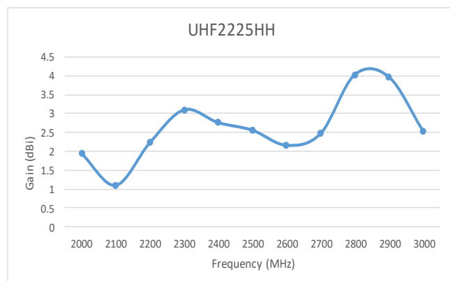
Gain (dBi)
