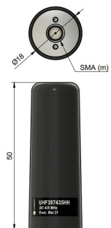
Outline Dimensions (mm)
