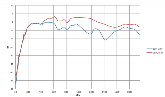
Gain (dBi)
